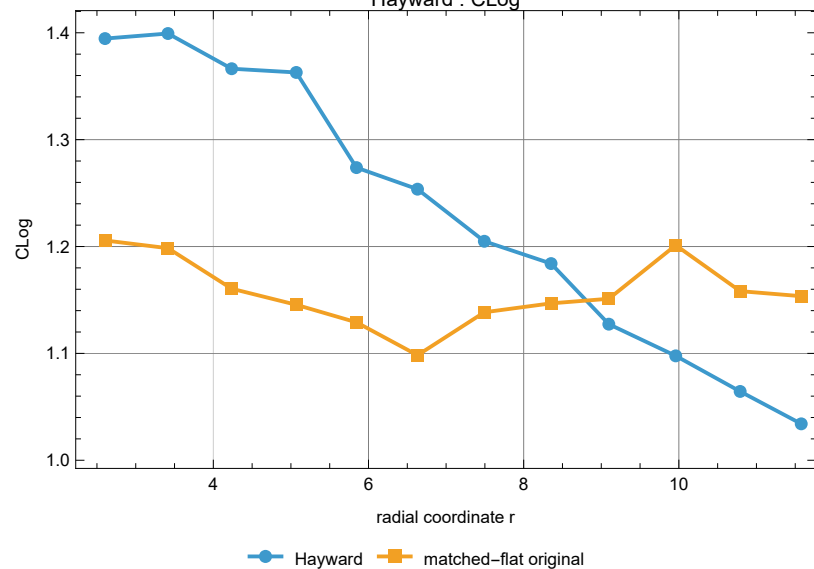
Hayward : CLog
