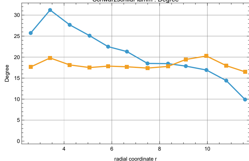
SchwarzschildFlamm : Degree
