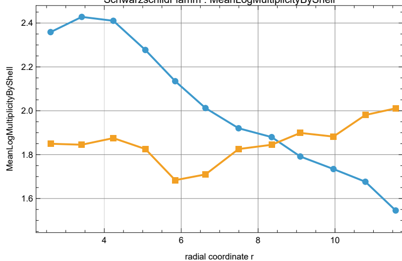
SchwarzschildFlamm : MeanLogMultiplicityByShell
