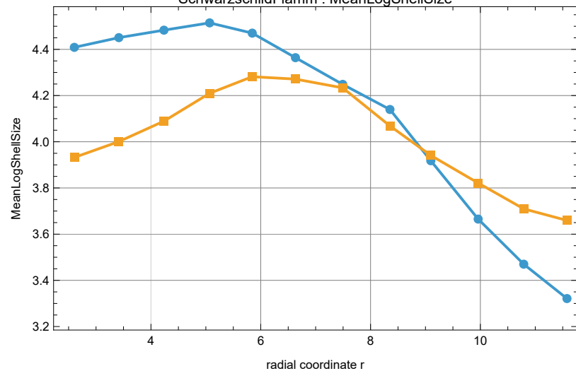
SchwarzschildFlamm : MeanLogShellSize
