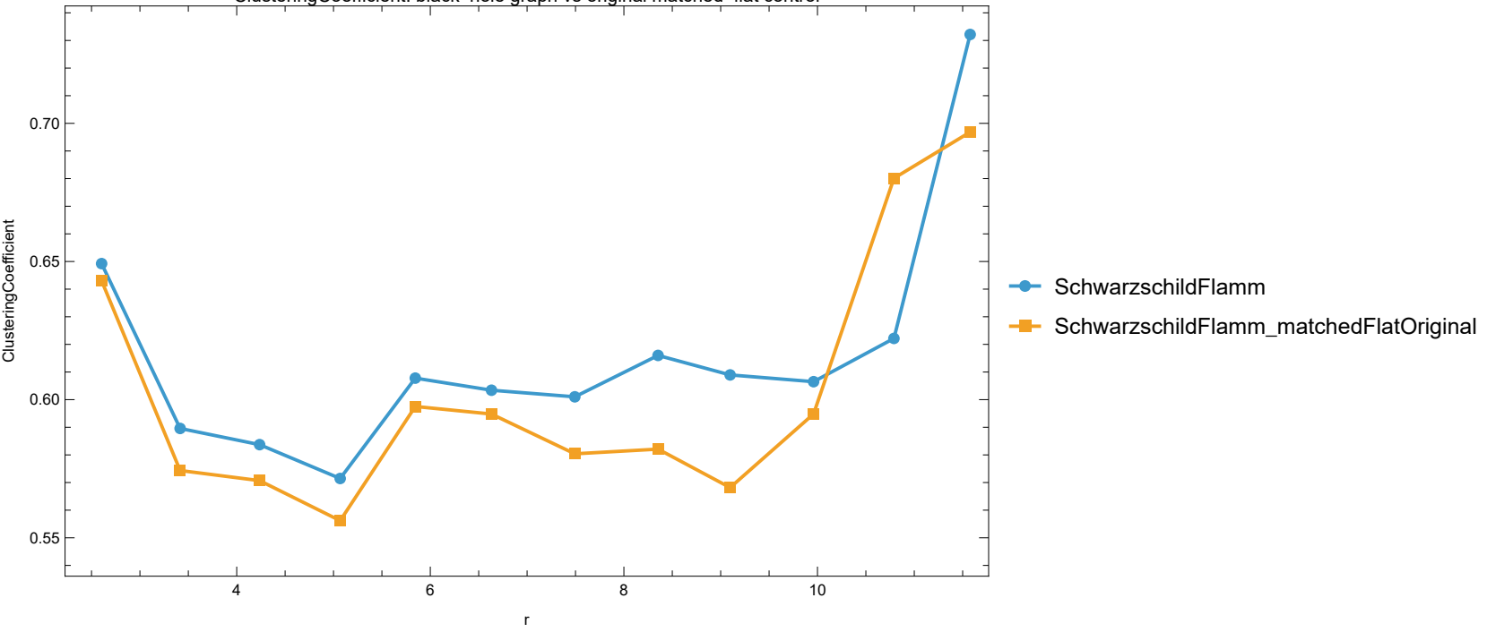
ClusteringCoefficient: black-hole graph vs original matched-flat control
