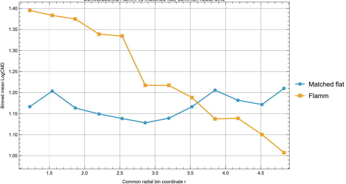
Schwarzschild/Flamm vs matched flat, common radial bins
