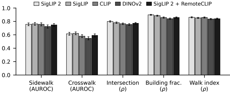
Zero-shot score on Pittsburgh
