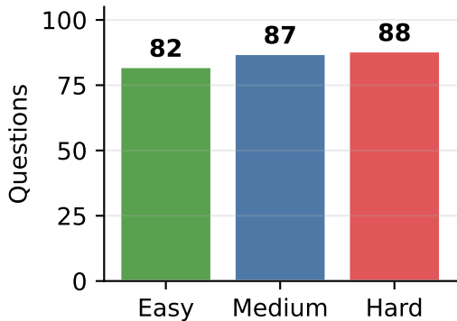
Difficulty Split
