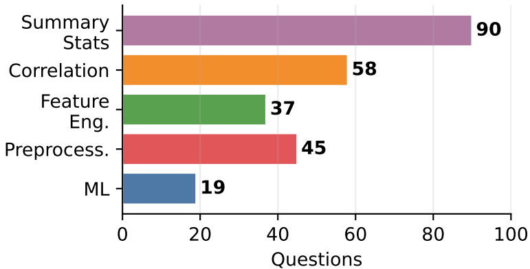
Annotated Concepts
