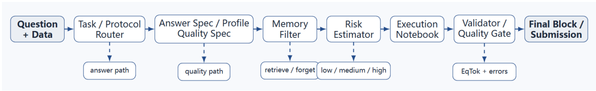
Figure 1: Integrated Resource-Aware DatawiseAgent architecture. The pipeline proceeds from question ingestion through task routing, answer specification, memory filtering, risk estimation, notebook execution, validation, and final submission. Each stage’s processing tier is determined by the risk estimator based on question difficulty, concept complexity, and verification history.
