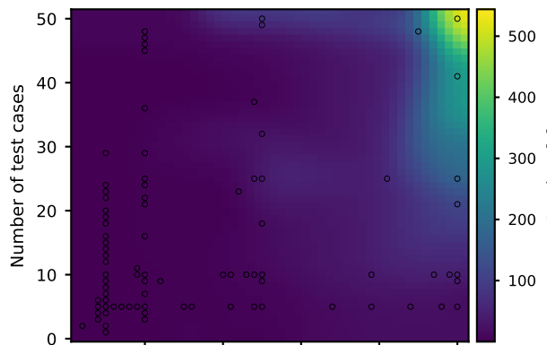
Runtime
