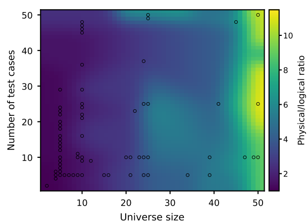
Physical/logical ratio
