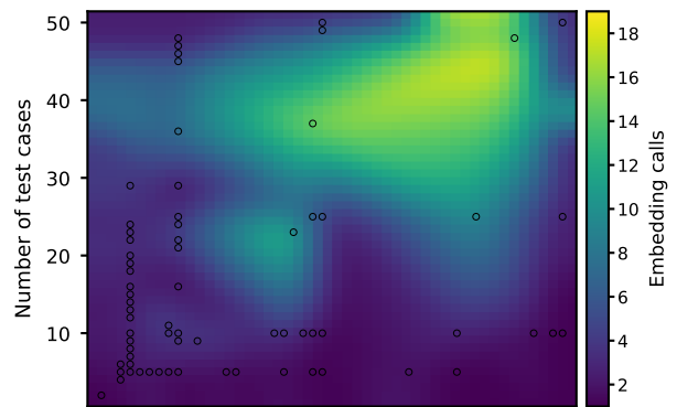
Embedding calls
