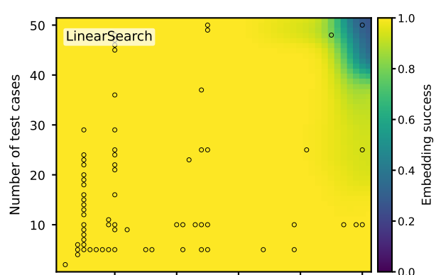
Embedding success
