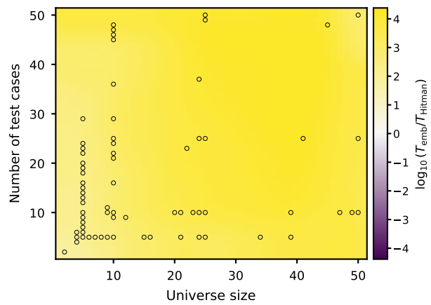
Emb./Hitman runtime
