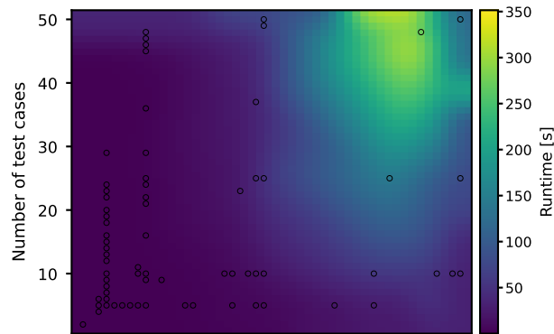
Runtime
