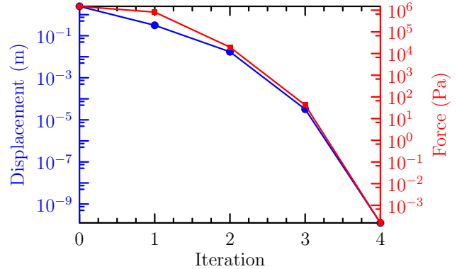
(b) Displacement and sum of forces on node C
