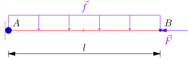
Figure 3: 1D Finite Element
