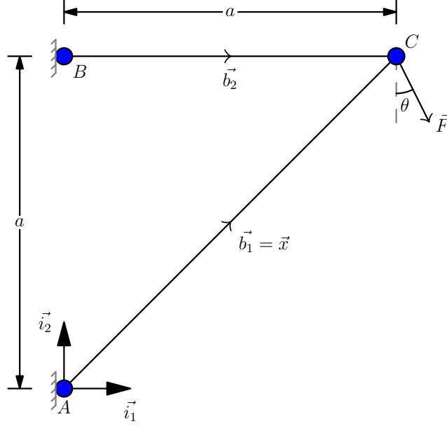
Figure 1: Two elements truss: console 2D
