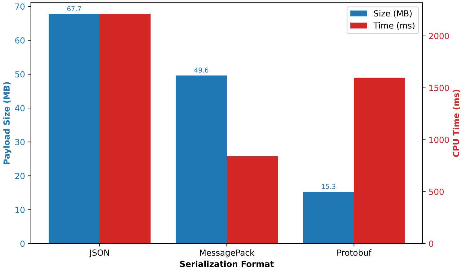
Serialization Performance: 1,000,000 Business Events
