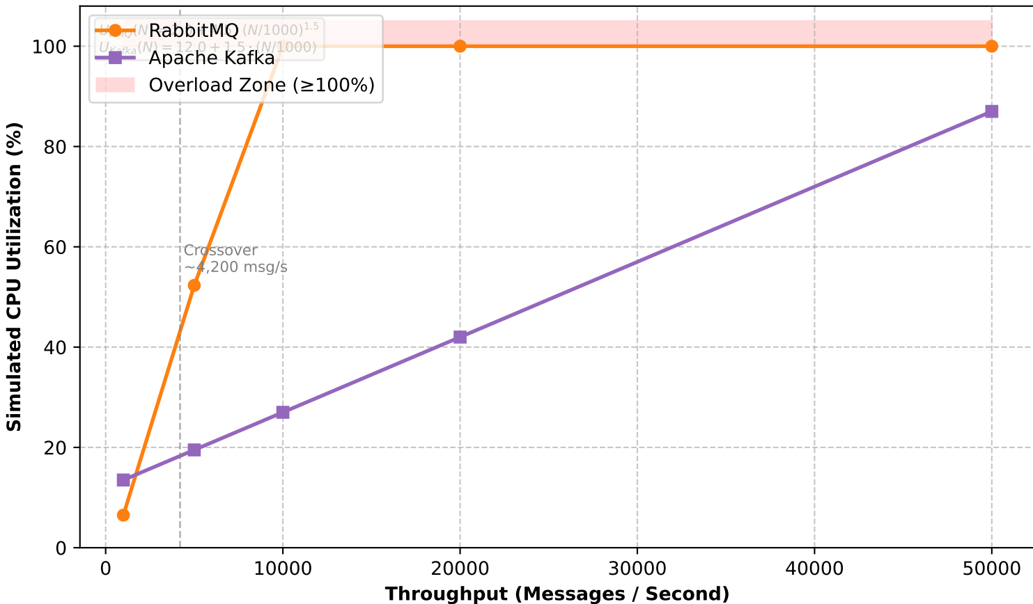
Message Broker CPU Overhead vs. Throughput (Mathematical Model)
