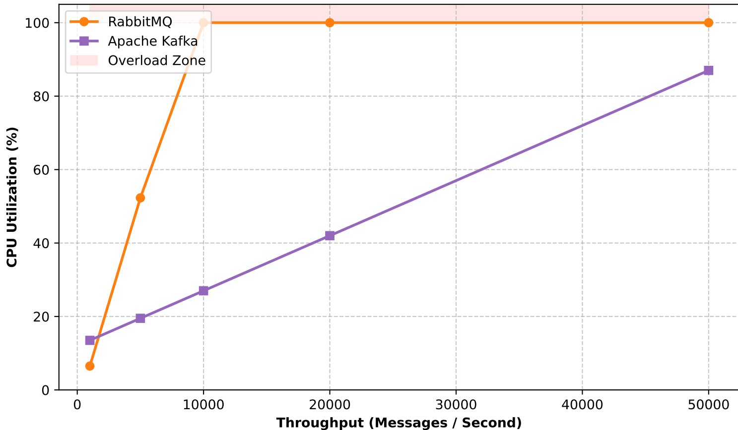
Message Broker CPU Overhead vs. Throughput
