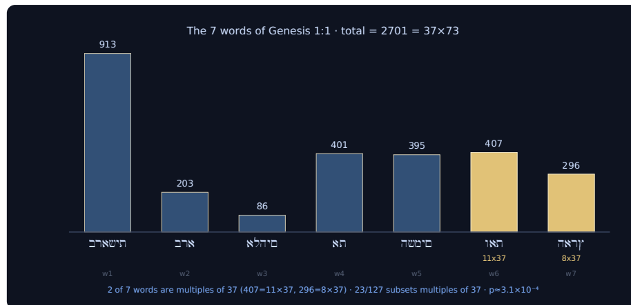
Fig. 10. The 7 words of Genesis 1:1 and their gematrias (913, 203, 86, 401, 395, 407, 296 = 2701 = 37×73). The two gold bars are the words that are multiples of 37 — the last two, (37×11=407) ואת, האו and (37×8=296) ינראה. A permutation null of the 28-letter multiset shows this bias is real: 23 of 127 non-empty subsets are multiples of 37 ( p \approx 3.1 \times 10^{-4} ) and 2/7 words ( p \approx 8.2 \times 10^{-3} ), beyond the trivial total 2701=37×73.
