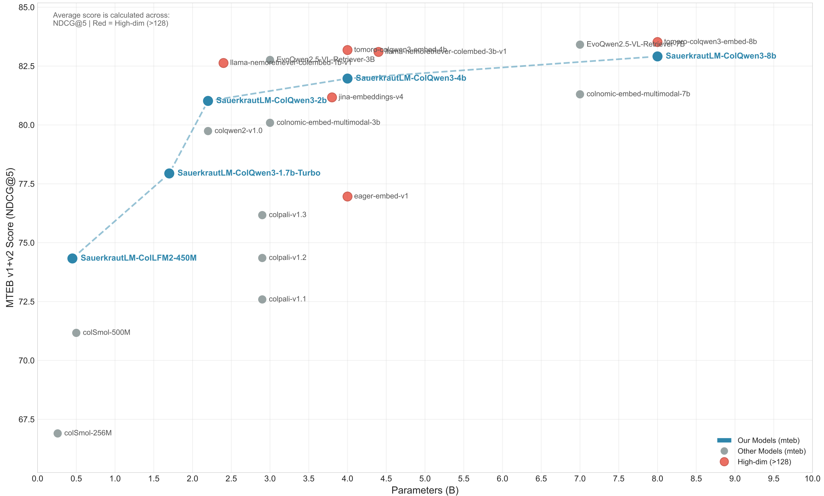
MTEB v1+v2: 128-dim vs High-dim Models
