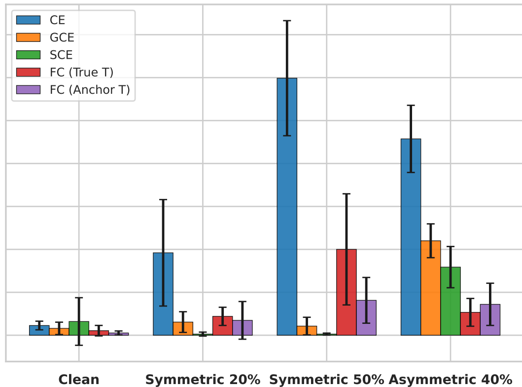
(A) Memorization Decay across Regimes
