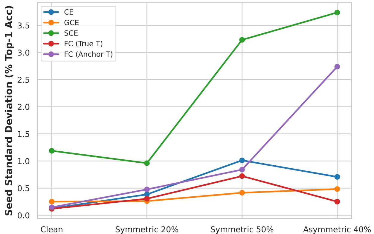
(B) Seed Variability across Regimes (N=3)
