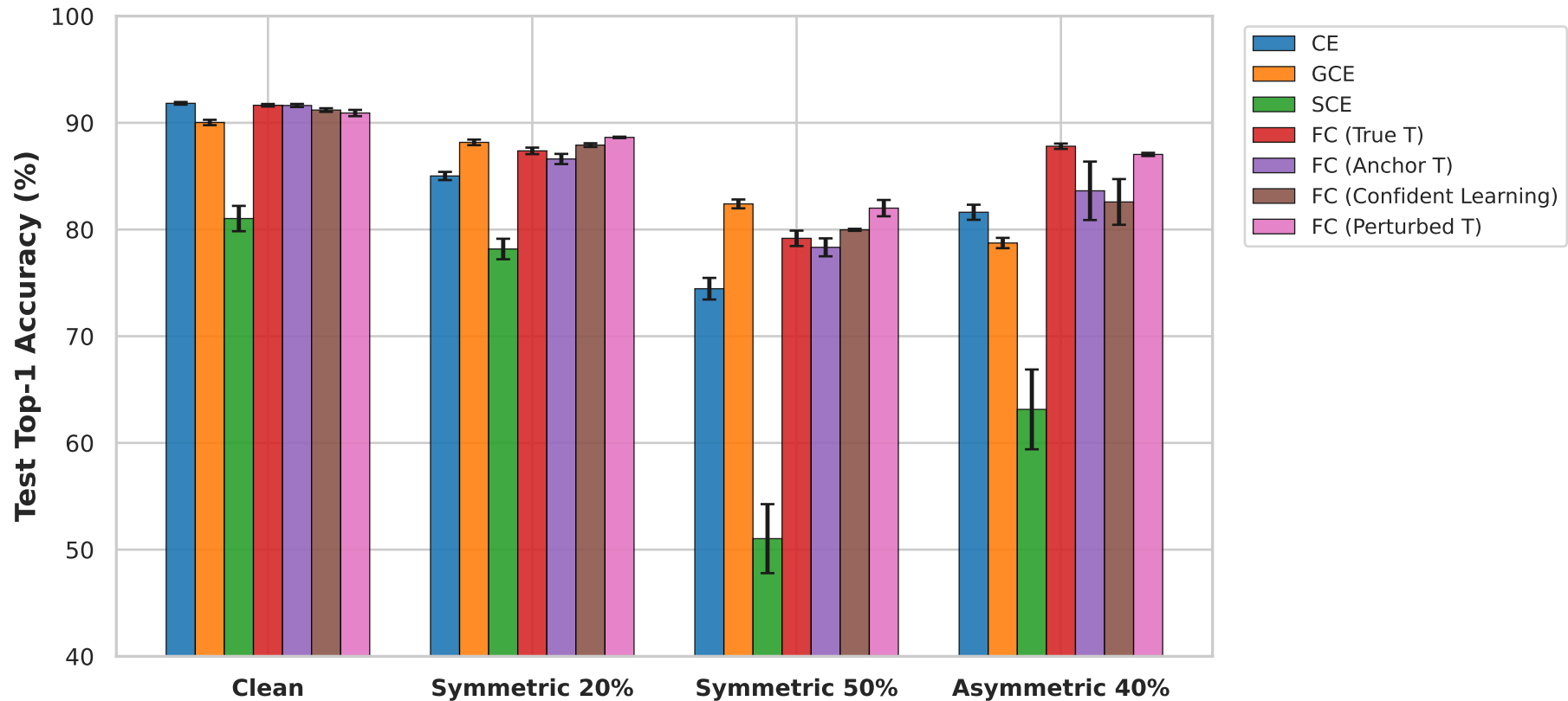
Figure 1: Test Top-1 Accuracy across Noise Regimes (Mean \pm SD, N=3 seeds)
