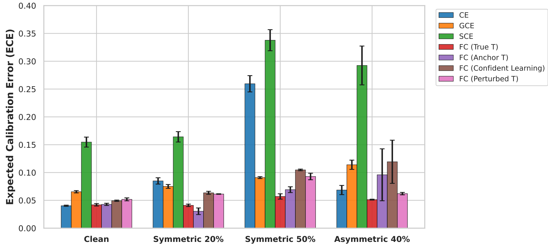
Figure 2: Expected Calibration Error (ECE) across Noise Regimes (Mean \pm SD)
