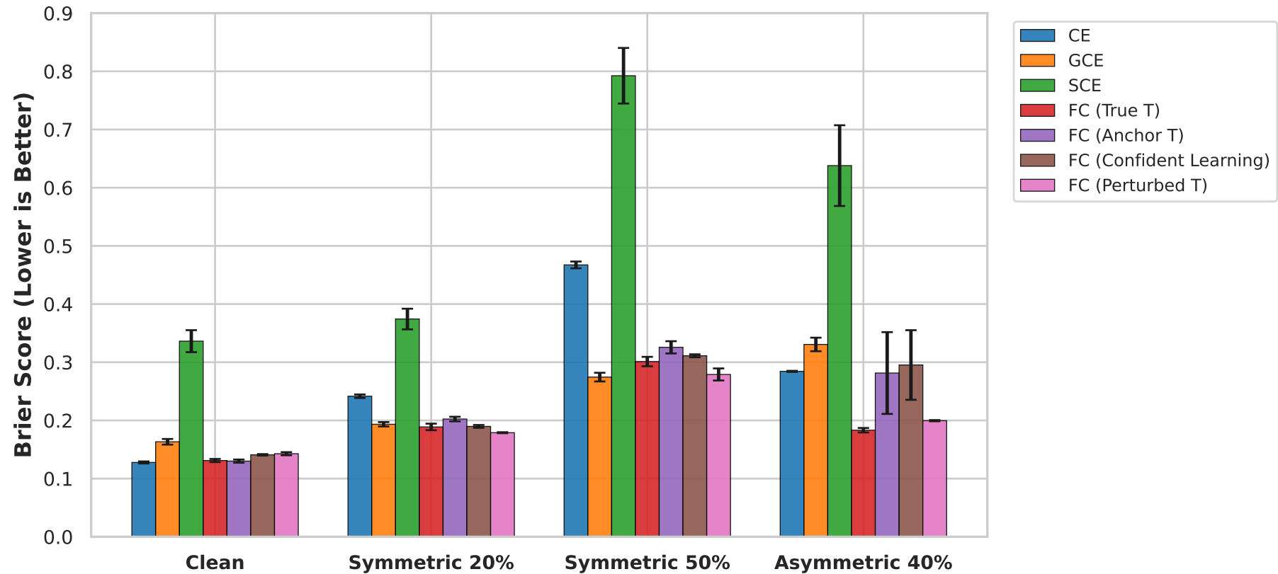
Figure 3: Brier Score across Noise Regimes (Mean \pm SD)
