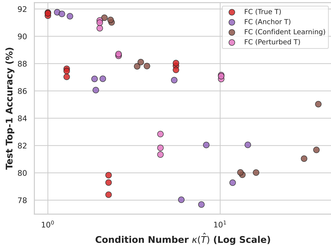
Figure 6: Accuracy vs Transition Matrix Condition Number \kappa(\hat{T})
