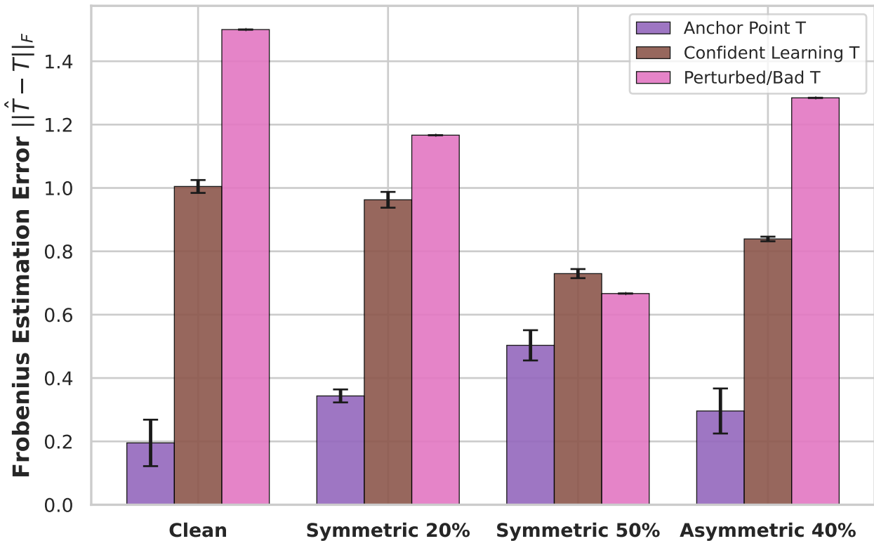
Figure 4: Transition Matrix Estimation Error ||\hat{T} - T||_F across Noise Regimes
