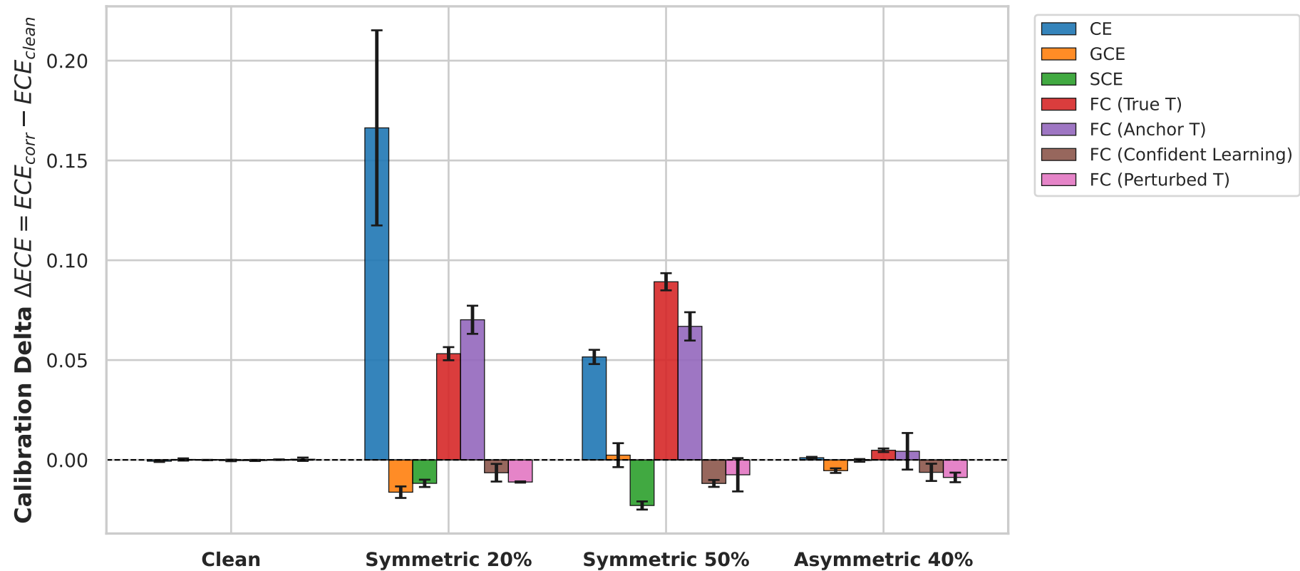
Figure 8: Corrupted Validation Calibration Penalty \Delta ECE (H3 Test)
