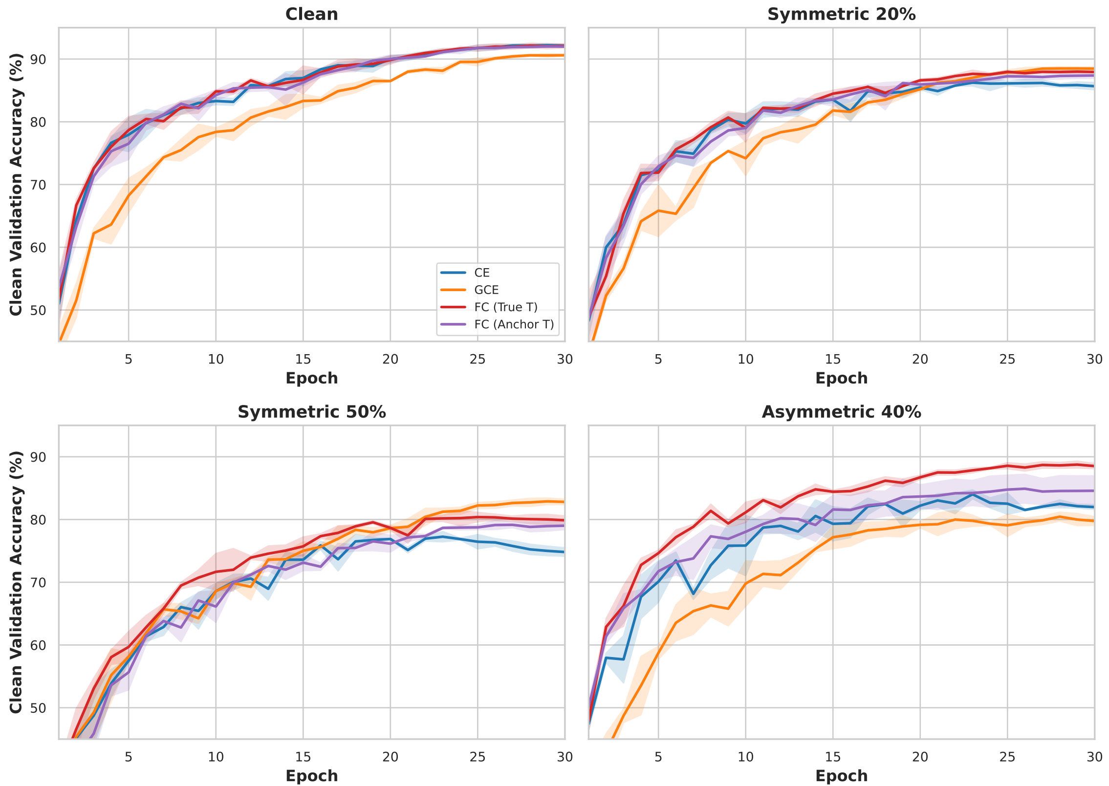
Figure 9: Clean Generalization Dynamics & Memorization Decay over 30 Epochs (H2 Test)
