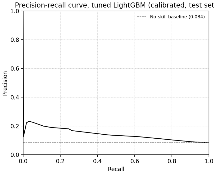
Figure 3: Precision-recall curve, tuned LightGBM, isotonic-calibrated, test set.
