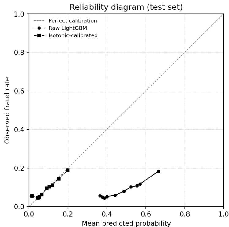
Figure 2: Reliability diagram, test set. Raw scores cluster between 0.35 and 0.65 regardless of true risk; calibrated scores track the diagonal down to the true base rate.
