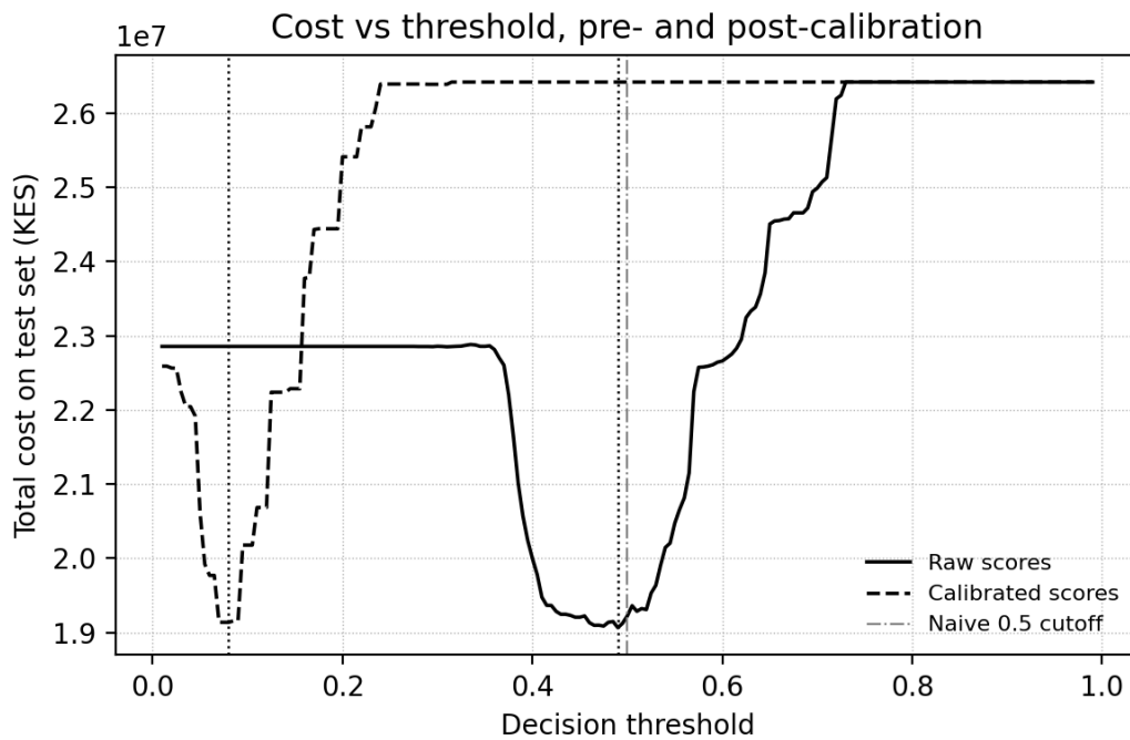
Figure 1: Total test-set cost as a function of the decision threshold, before and after isotonic calibration. Vertical dotted lines mark each curve's own cost-minimising threshold; the dash-dot line marks the naive 0.5 cutoff.
