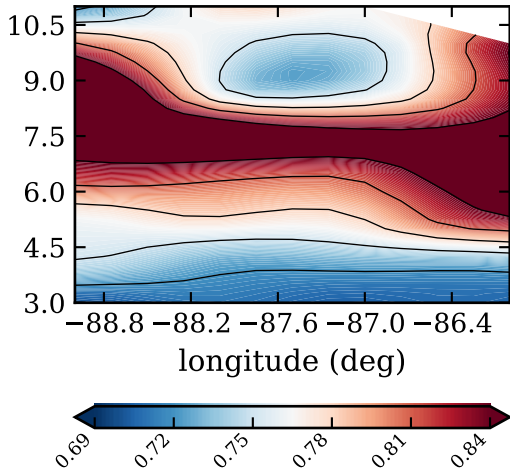
RF01, day 219, satfrac
