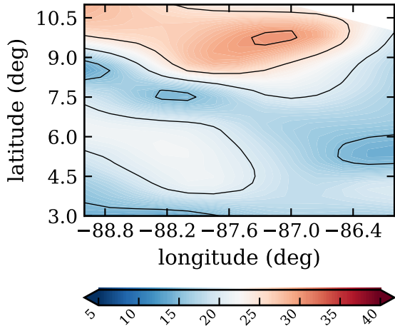
RF01, day 219, instab index (J/K/kg)
