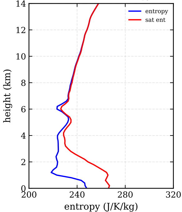
RF01: 3DVAR (-88.5, 8.5) - entropy / sat ent
