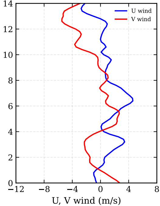
RF01: 3DVAR (-88.5, 8.5) - U wind / V wind
