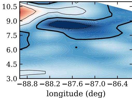
RF01, day 219, srcent ( \text{W/m}^2 )
