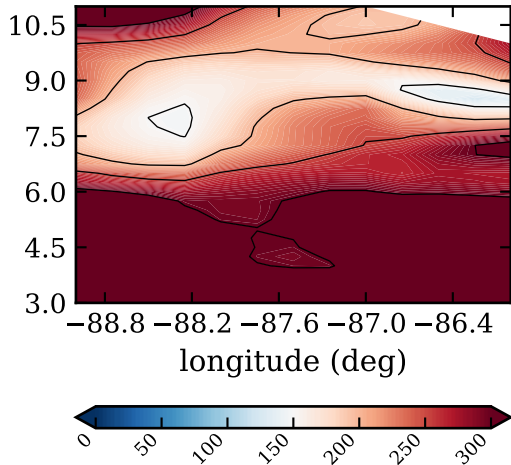
RF01, day 219, eflux (W/m 2 )
