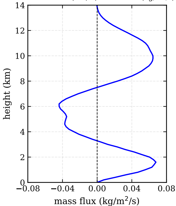
RF02: 3DVAR (-78, 5) - mass flux ( \text{kg/m}^2/\text{s} )
