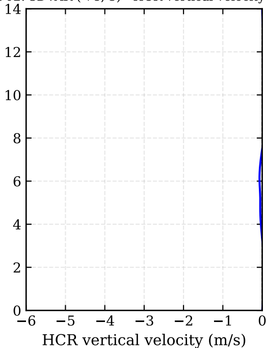
RF02: 3DVAR (-78, 5) - HCR vertical velocity (m/s)
