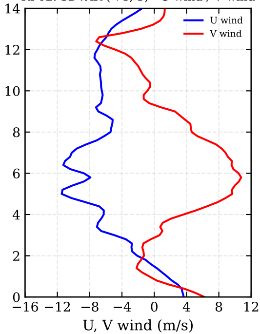
RF02: 3DVAR (-78, 5) - U wind / V wind
