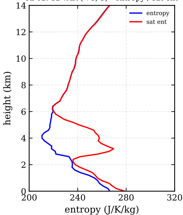
RF02: 3DVAR (-78, 5) - entropy / sat ent
