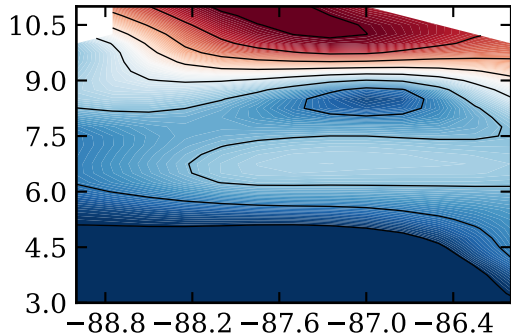
RF03, day 224, instab index (J/K/kg)
