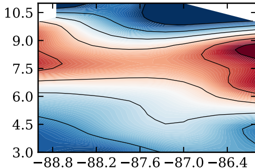
RF03, day 224, satfrac
