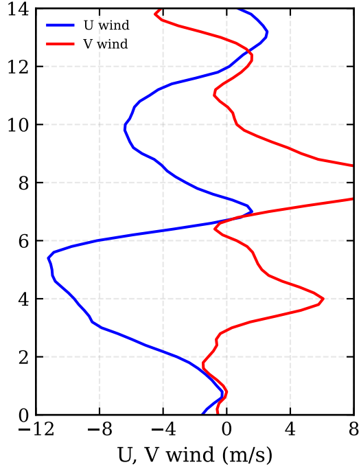
RF03: 3DVAR (-88.5, 8.5) - U wind / V wind
