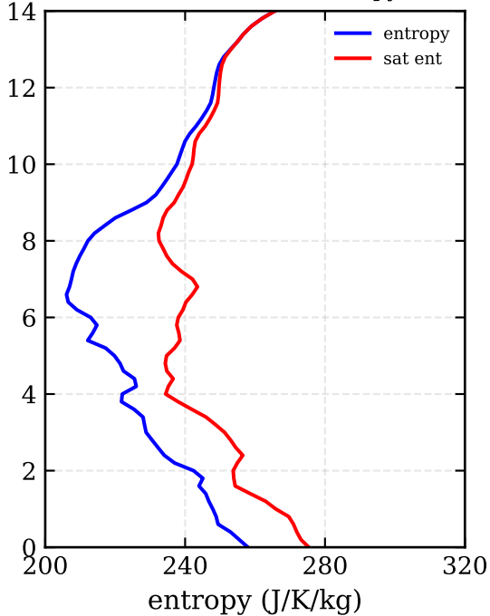
RF03: 3DVAR (-88.5, 8.5) - entropy / sat ent
