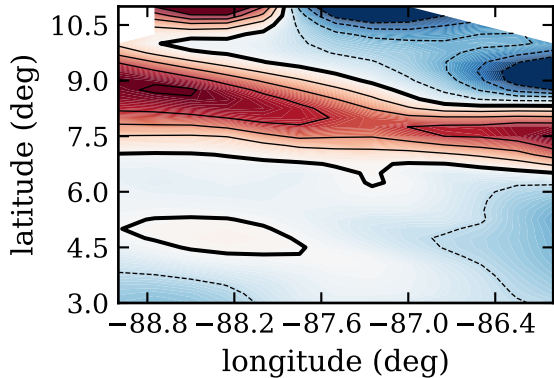
RF03, day 224, srcmr, ( \text{W/m}^2 )
