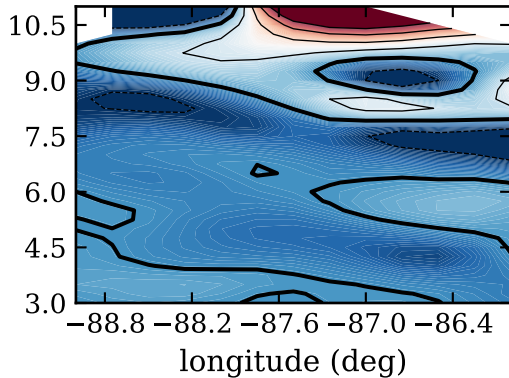
RF03, day 224, srcent ( \text{W/m}^2 )
