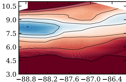
RF03, day 224, eflux (W/m 2 )
