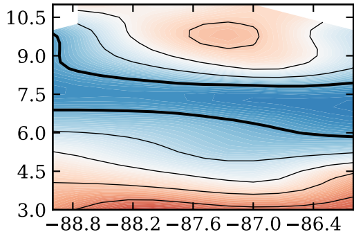
RF03, day 224, dcin, (J/K/kg)
