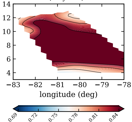
RF04c, day 228, satfrac
