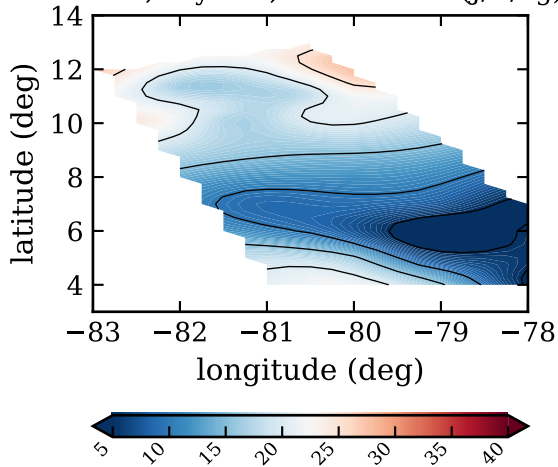
RF04c, day 228, instab index (J/K/kg)
