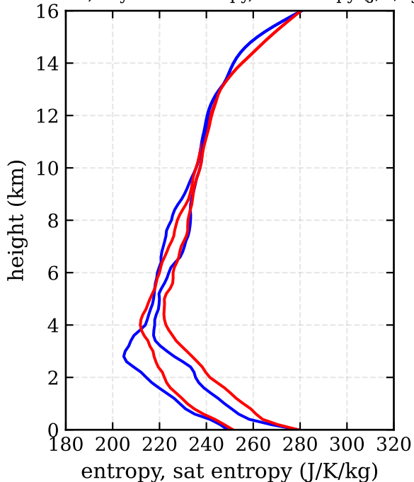
RF04c, day 228 - entropy, sat entropy (J/K/kg)
