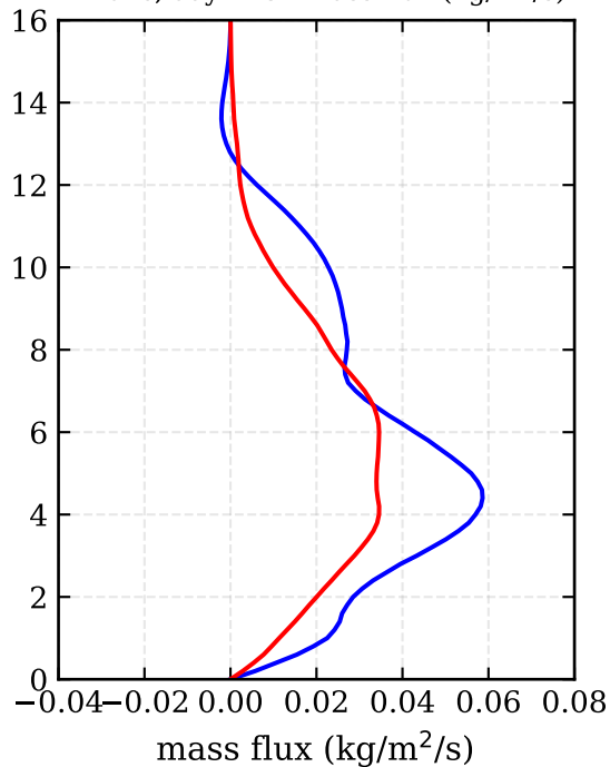
RF04c, day 228 - mass flux (kg/m 2 /s)
