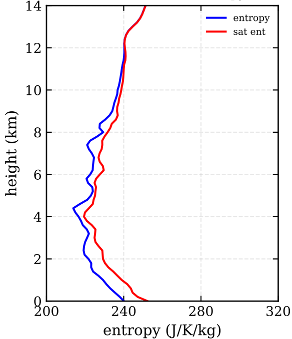
RF04c: 3DVAR (-78.5, 6.3) - entropy / sat ent
