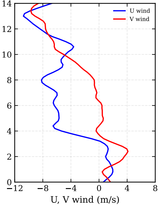
RF04c: 3DVAR (-78.5, 6.3) - U wind / V wind
