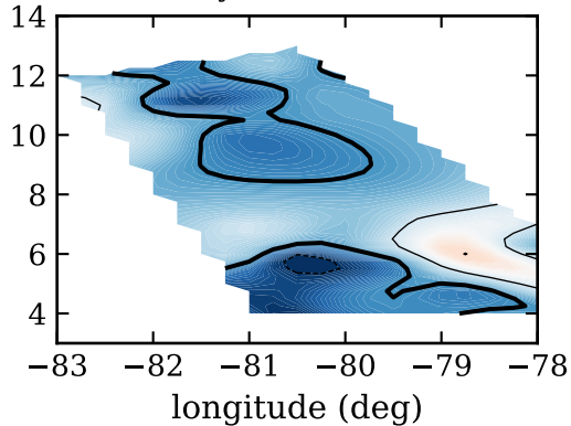
RF04c, day 228, srcent ( \text{W/m}^2 )
