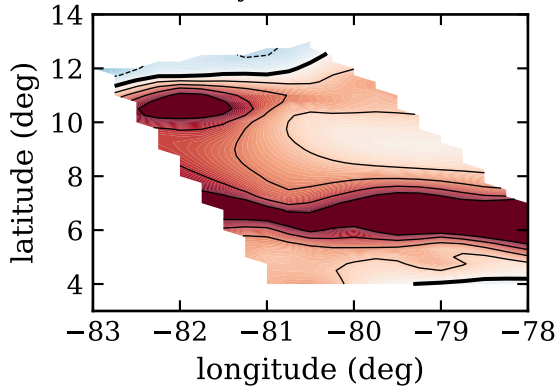
RF04c, day 228, srcmr, ( \text{W/m}^2 )
