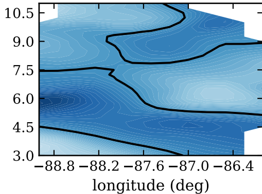
RF05, day 229, srcent ( \text{W/m}^2 )
