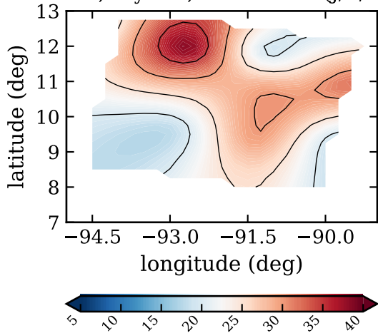
RF06, day 230, instab index (J/K/kg)
