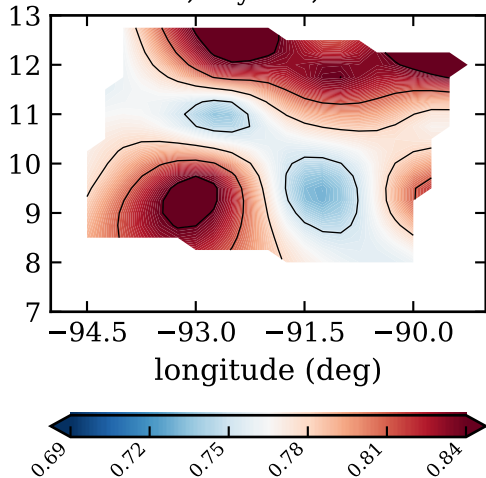
RF06, day 230, satfrac
