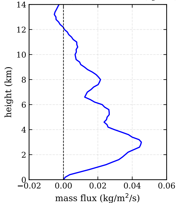
RF06: 3DVAR (-93, 10) - mass flux ( \text{kg/m}^2/\text{s} )
