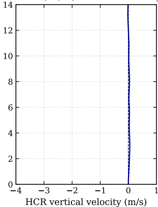
RF06: 3DVAR (-93, 10) - HCR vertical velocity (m/s)
