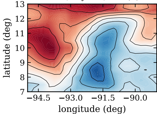
RF06, day 230, SST (C)
