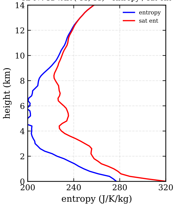
RF07: 3DVAR (-81, 11) - entropy / sat ent
