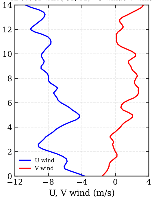
RF07: 3DVAR (-81, 11) - U wind / V wind
