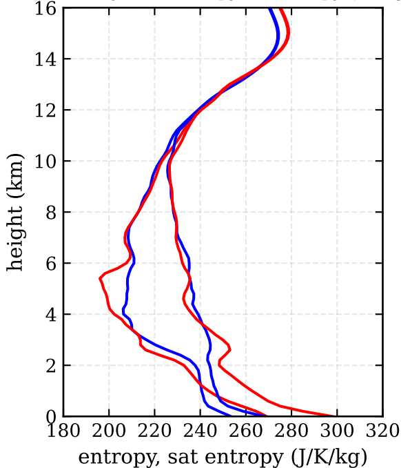
RF08, day 235 - entropy, sat entropy (J/K/kg)
