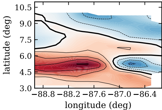
RF08, day 235, srcmr, ( \text{W/m}^2 )
