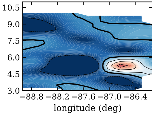
RF08, day 235, srcent ( \text{W/m}^2 )
