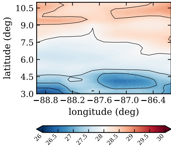
RF08, day 235, SST (C)
