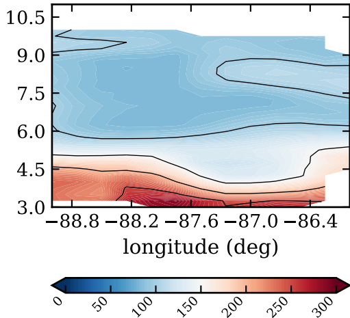
RF08, day 235, eflux (W/m 2 )
