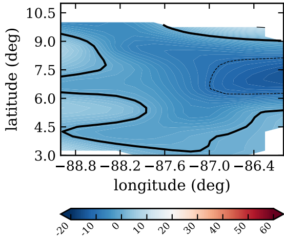
RF08, day 235, dcin, (J/K/kg)
